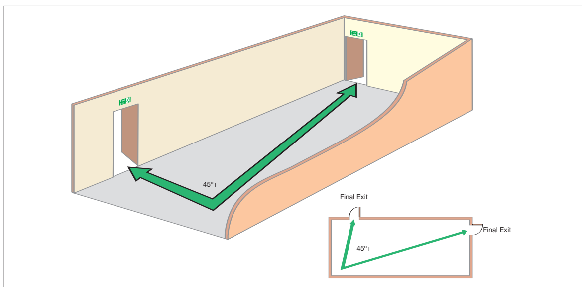
Figure 42: Ground floor premises with more than one exit
