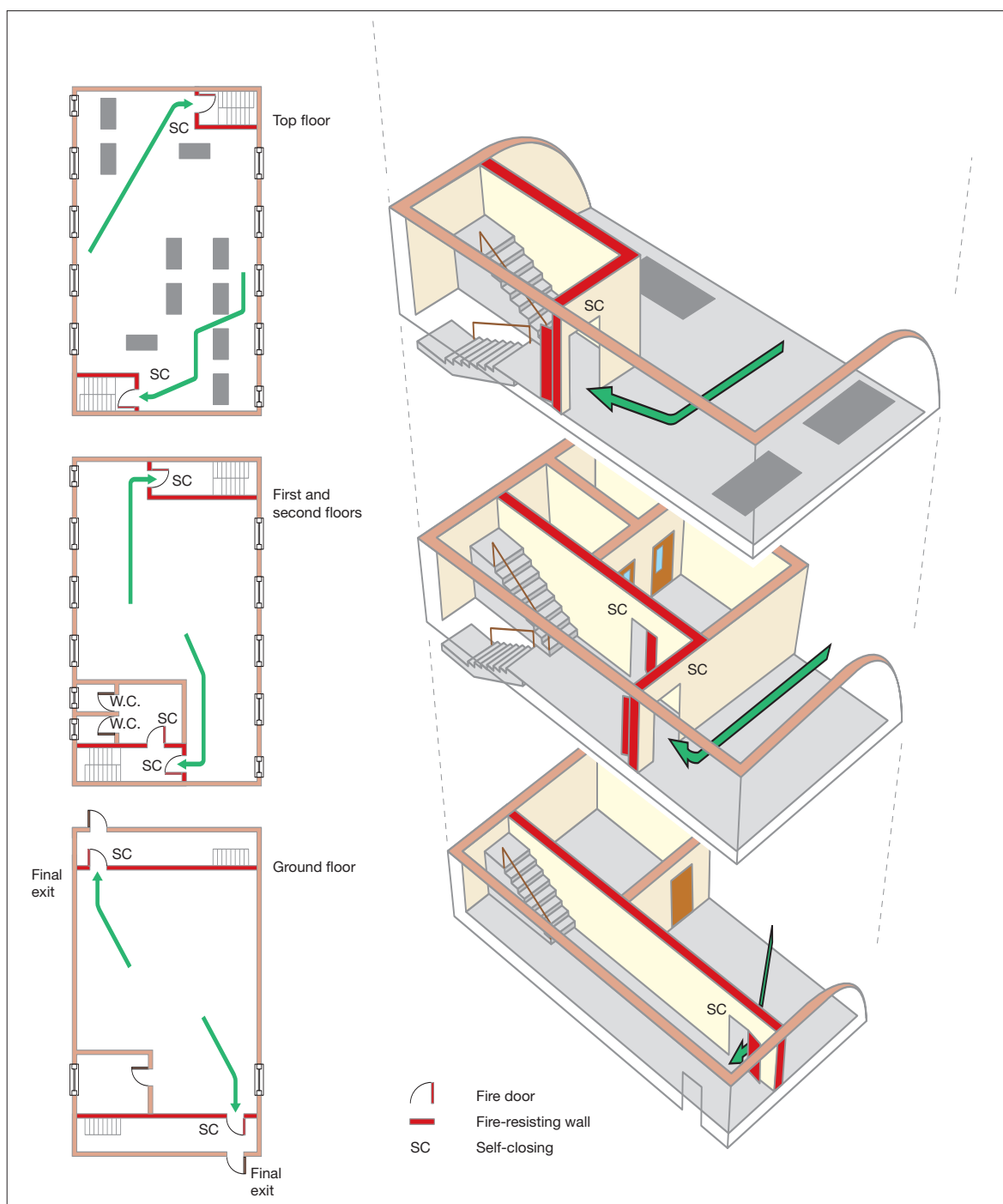
Figure 48: Four-storey premises, ground and up to three upper floors
