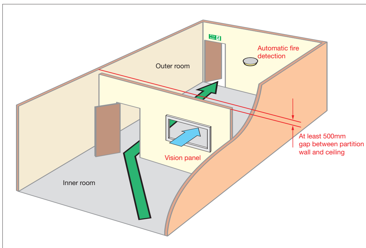
Figure 27: Inner rooms
