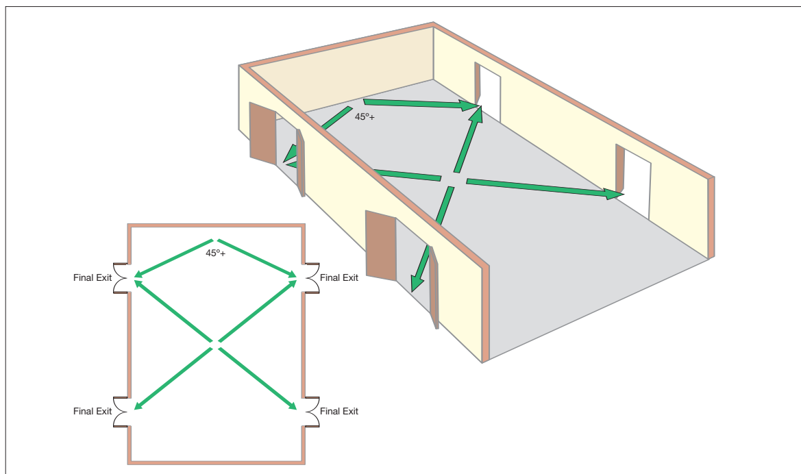
Figure 43: Ground floor premises with more than one exit
