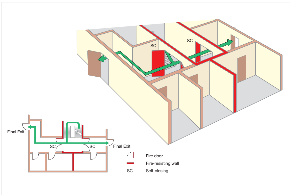
Figure 37: Example of two escape routes from a stairway to final exits
