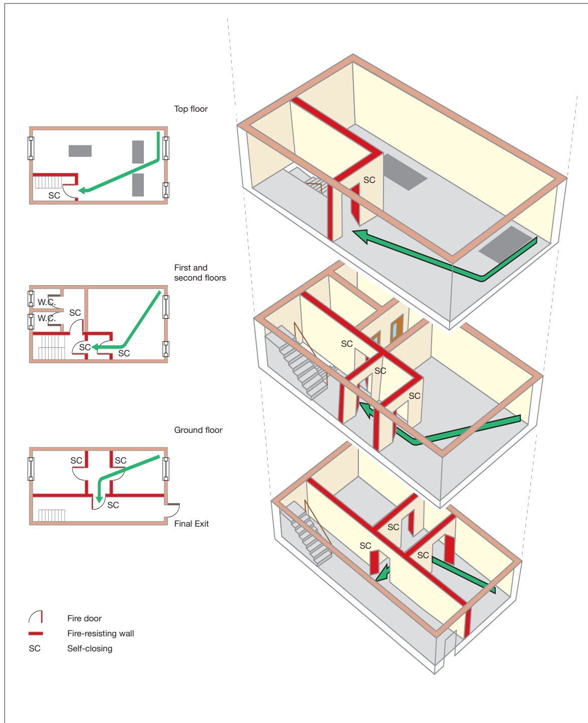
Figure 54: Four-storey, ground and up to three upper floors – protected by lobbies/corridors
