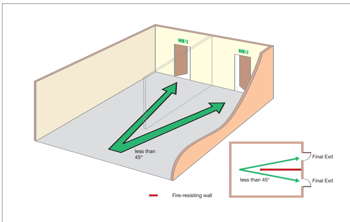
Figure 26: Alternative exits (separated by fire-resisting construction)
