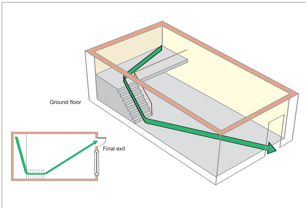
Figure 44: Ground floor premises with a single exit (including a mezzanine) (as part of larger premises)
