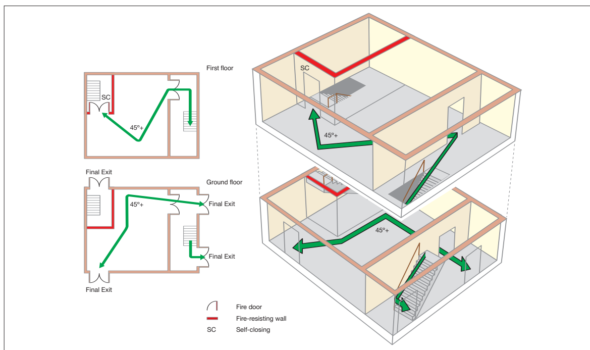
Figure 45: Two-storey premises: lower risk premises (e.g. church hall)
