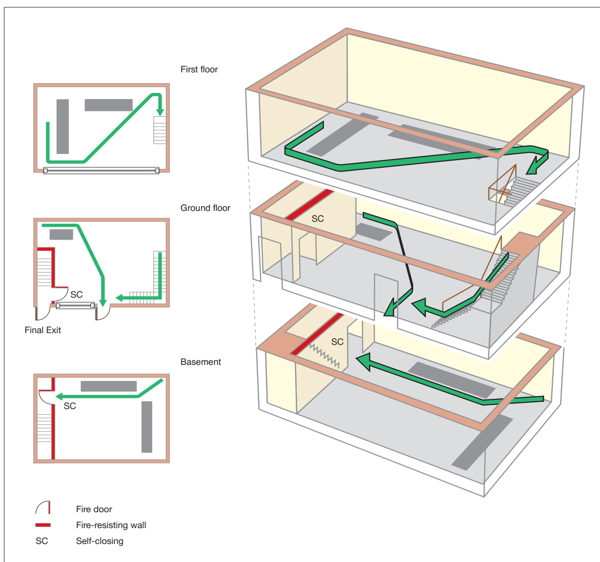
Figure 52: Three-storey premises, small basement, ground and one upper floor
