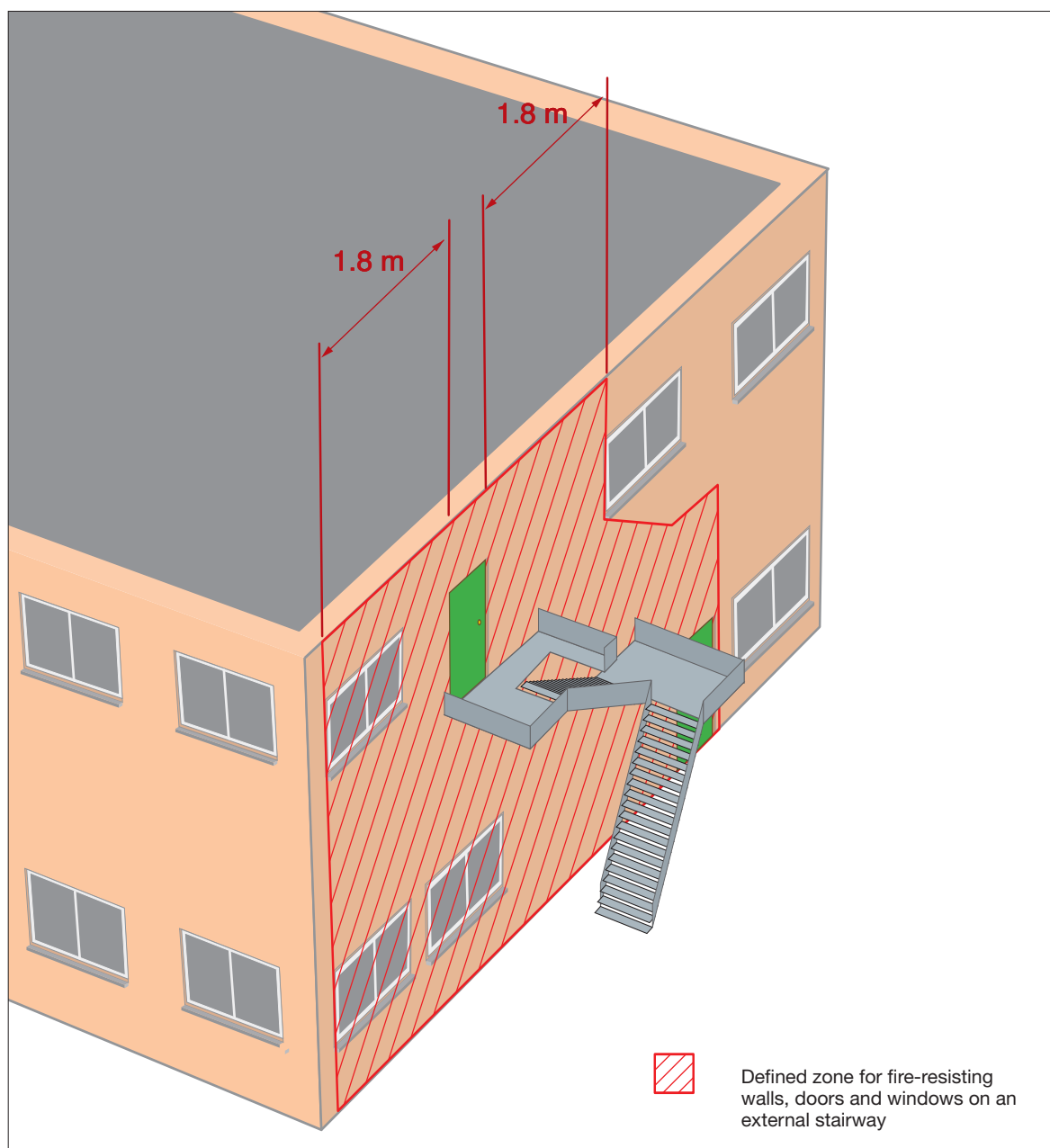
Figure 40: Protection to an external stairway
