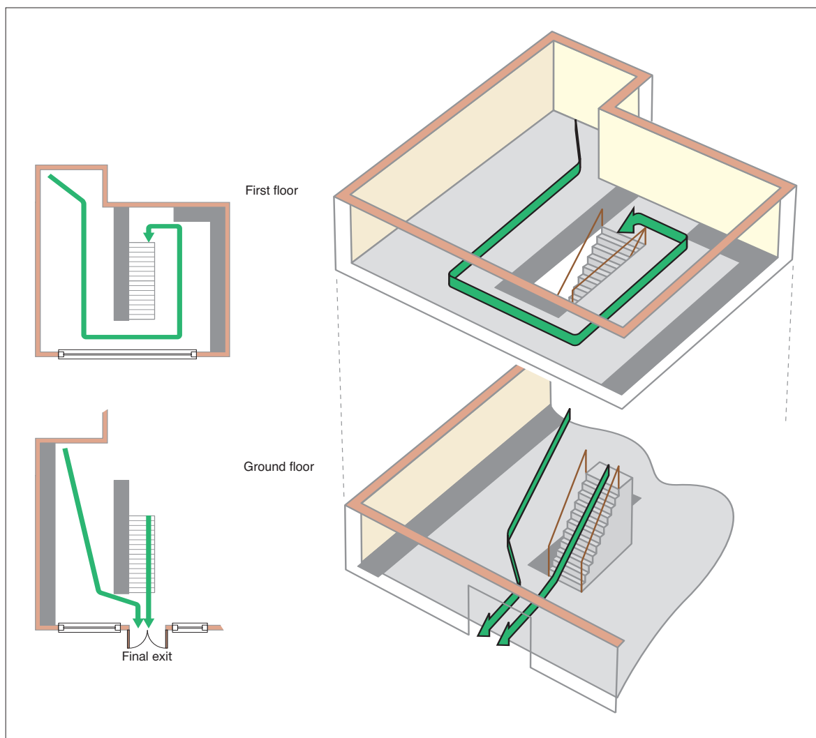
Figure 50: Two-storey premises, ground and one upper floor
