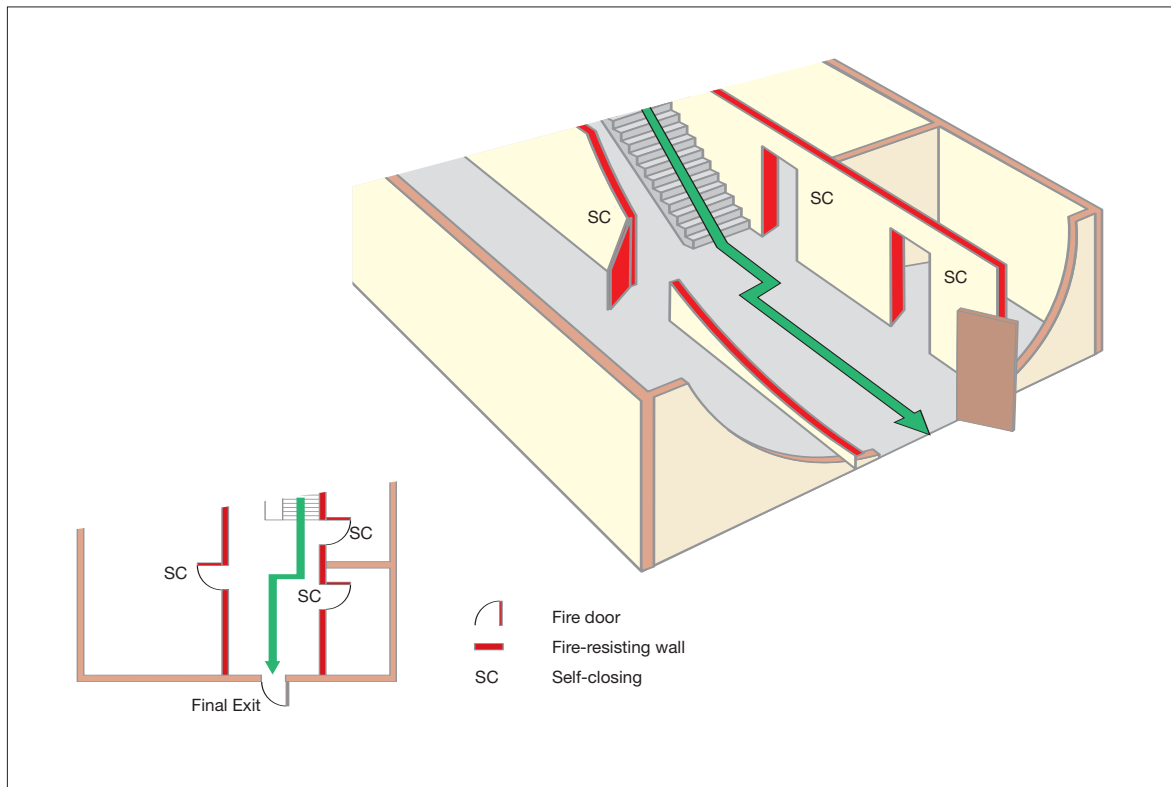
Figure 36: Examples of a protected route from a stairway to a final exit
