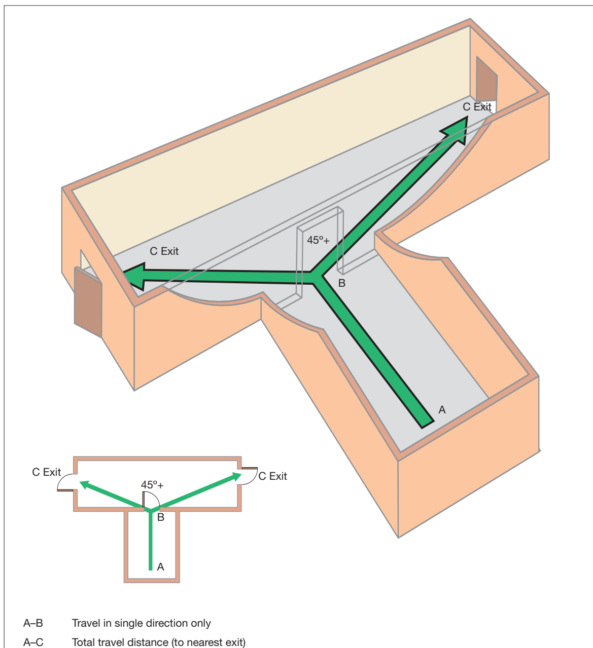
Figure 29: Measuring travel distance from initial dead end (inner room)
