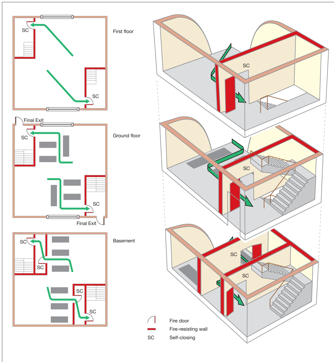
Figure 47: Three-storey premises, basement, ground and one upper floor
