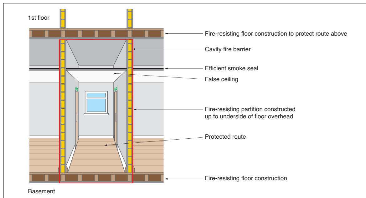
Figure 64: Fire-resisting construction
