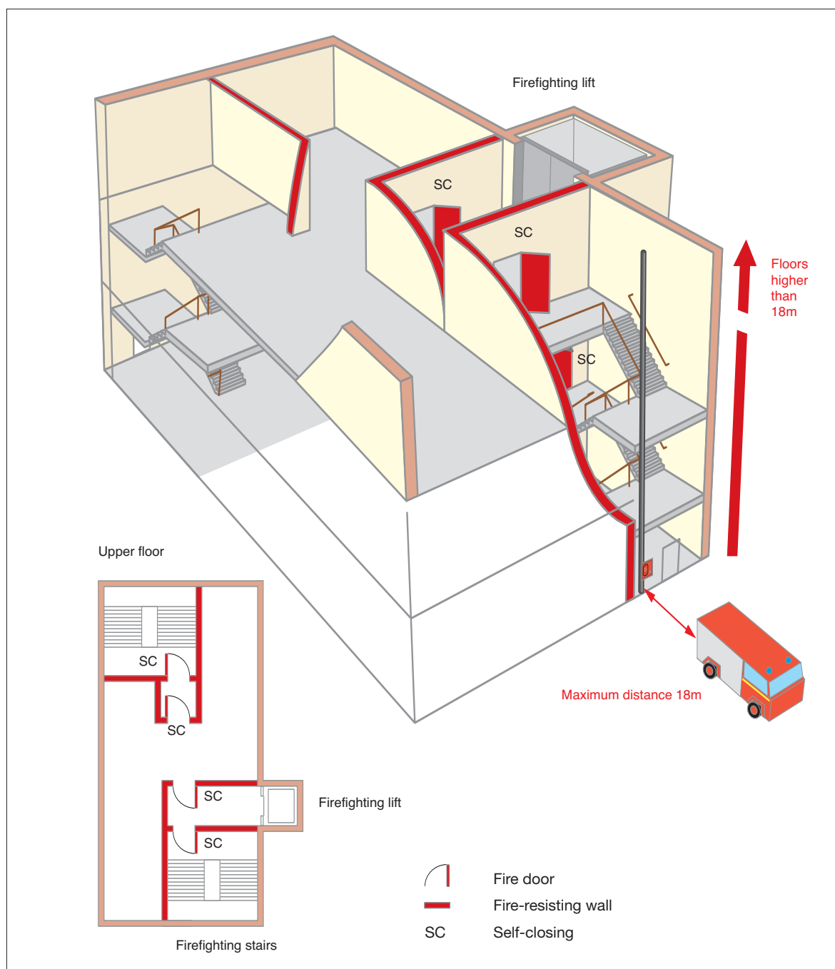
Figure 49: Tall building with a firefighting shaft
