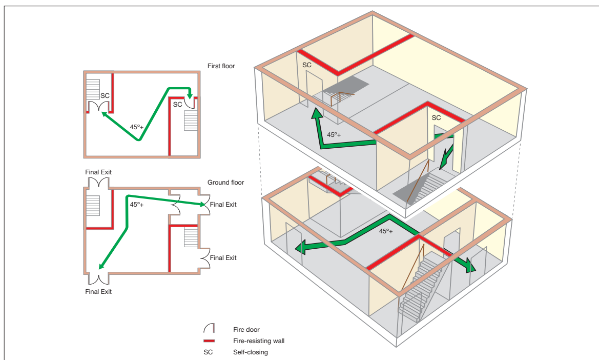
Figure 46: Two-storey premises: higher risk premises (e.g. nightclub)
