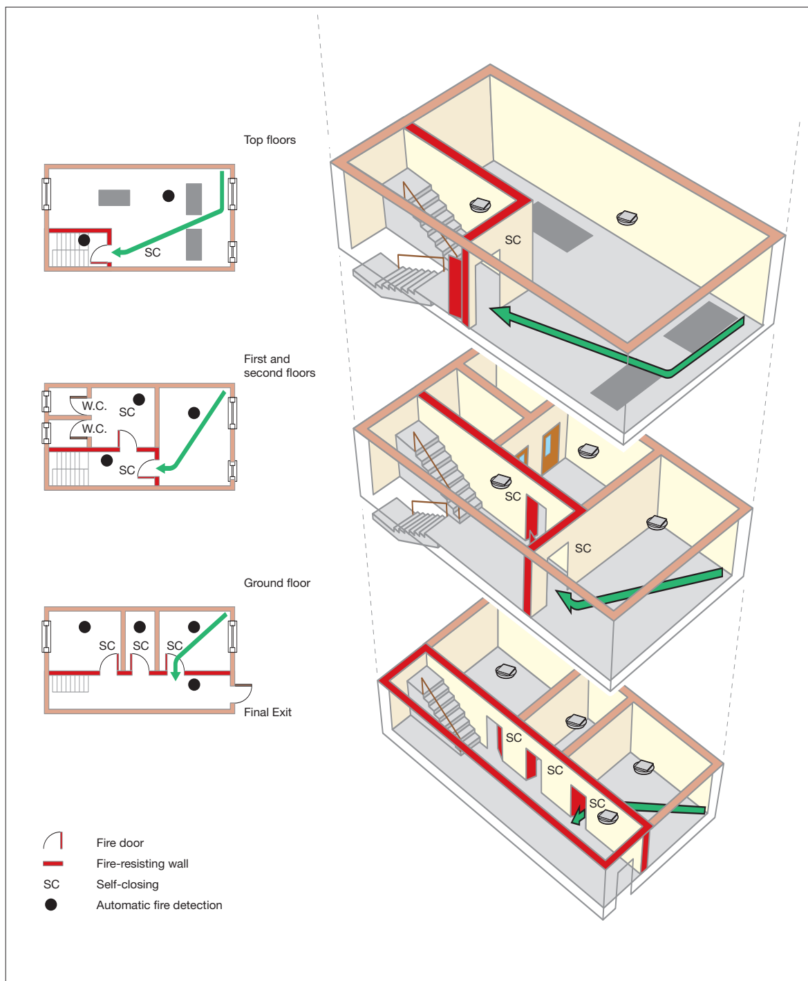
Figure 55: Four-storey, ground and up to three upper floors – protected with automatic fire detection
