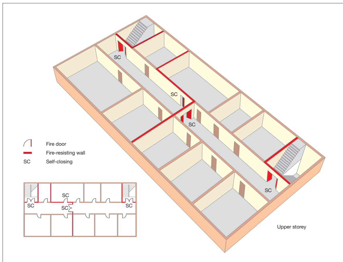
Figure 34: Subdivision of corridor between two stairways or exits
