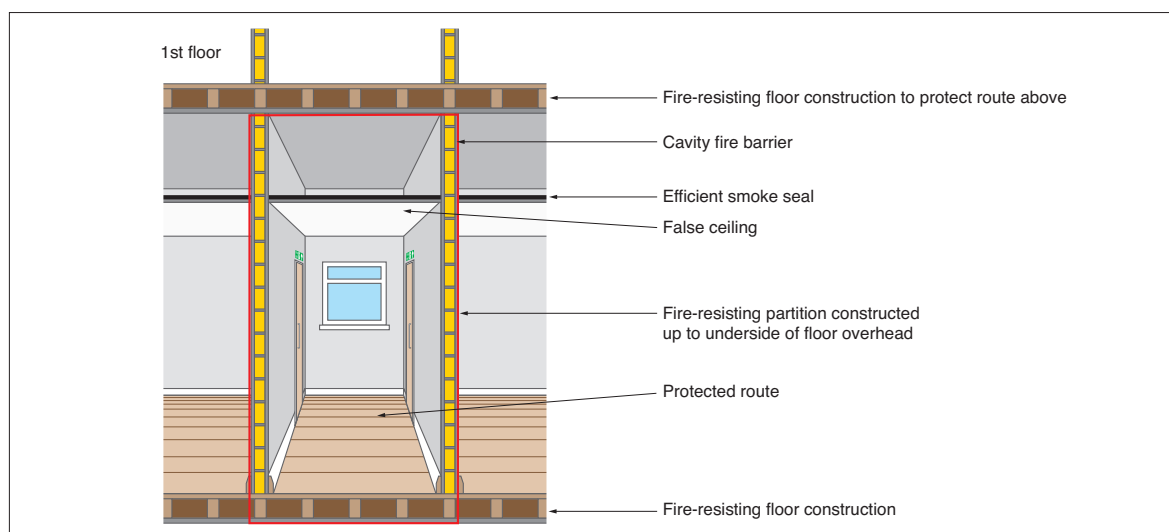
Figure 31: Fire-resisting construction
