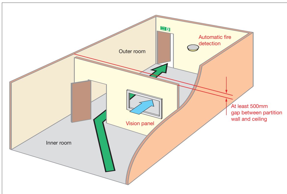
Figure 25: Inner rooms
