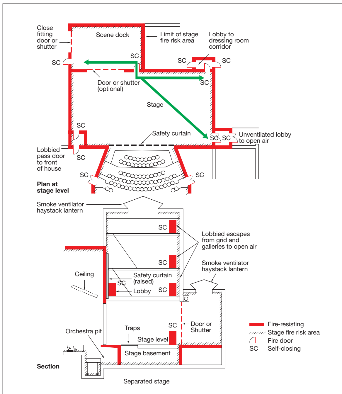
Figure 40: Example of exit arrangements – separated stage
