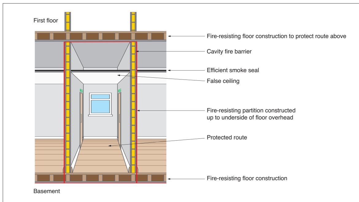
Figure 67: Fire-resisting construction
