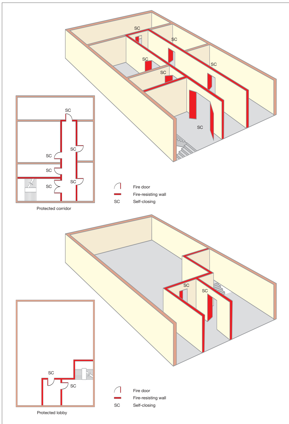
Figure 35: Examples of a stairway with protected lobby/corridor approach
